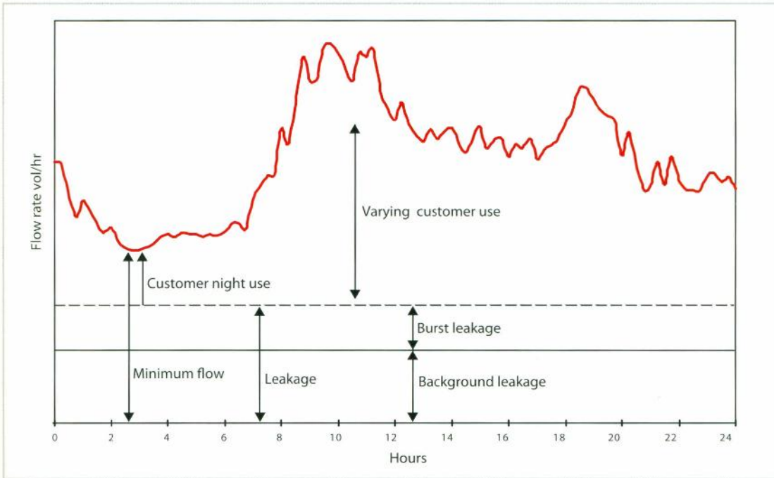
Figure 7.2: Typical 24-hour DMA flow profile
