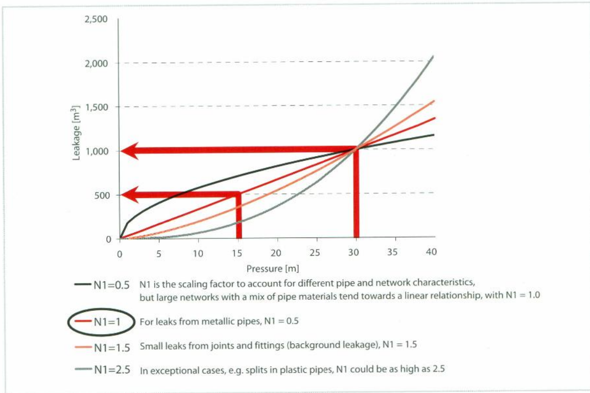
Figure 6.4: Pressure/leakage relationship
