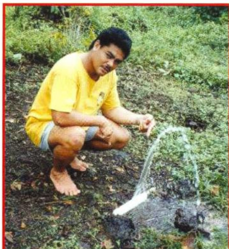
Typically more difficult to detect, service connection leaks result in significant water losses.
