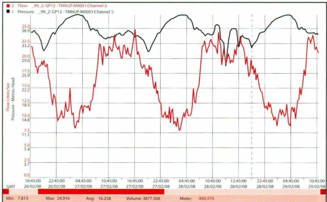
Figure 7.3: DMA flow and pressure relationship over a three-day period
